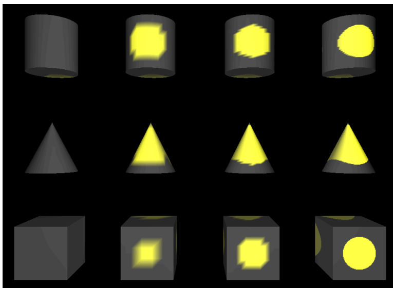
Figure 3.2. Different triangulations example (Gouraud shading)
